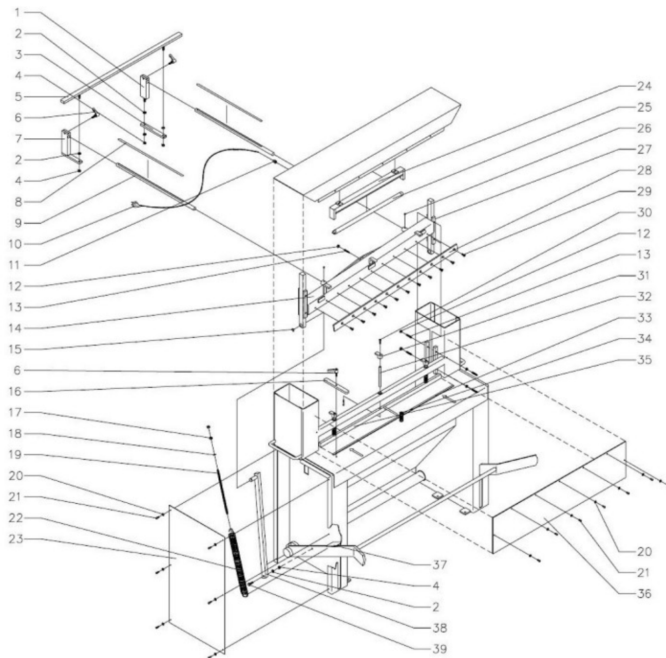
Abb. / Fig. 1: FTBS 1050-12 M und 1300-12 M / Spare parts drawing 1050-12 M and 1300-12 M
