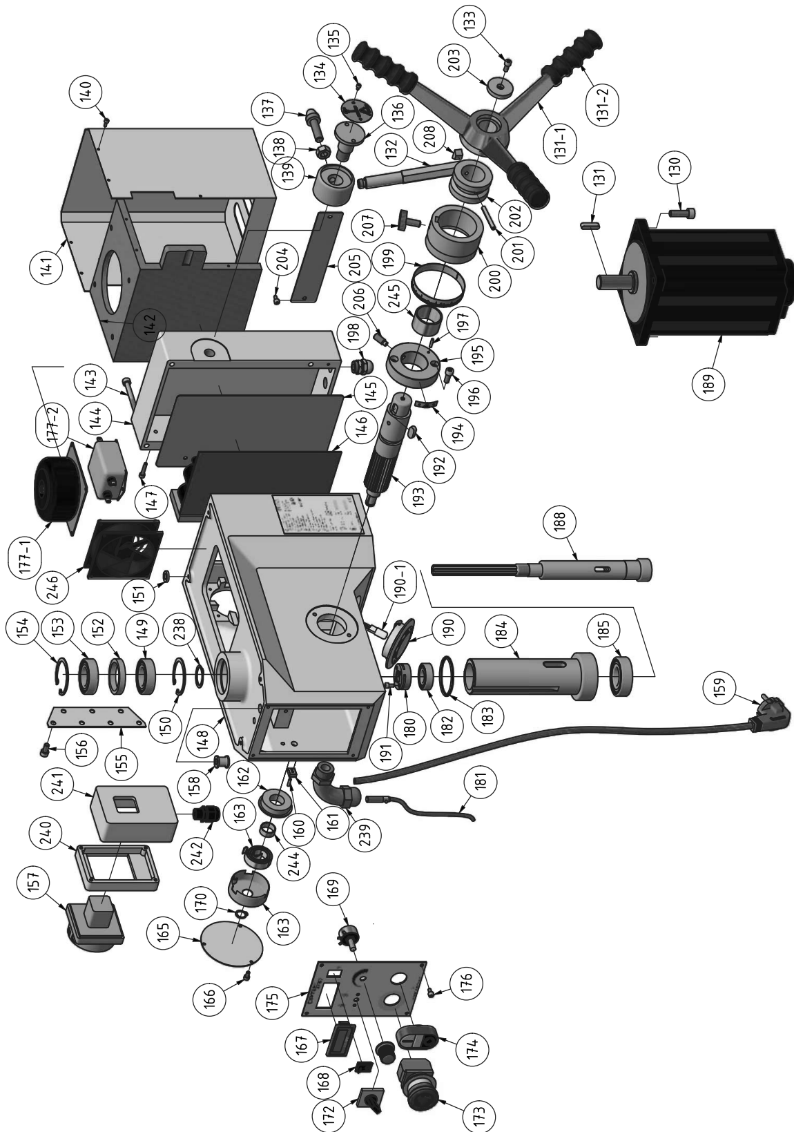
Img.1-4: Bohrkopf B24HV - Drilling head B24HV
