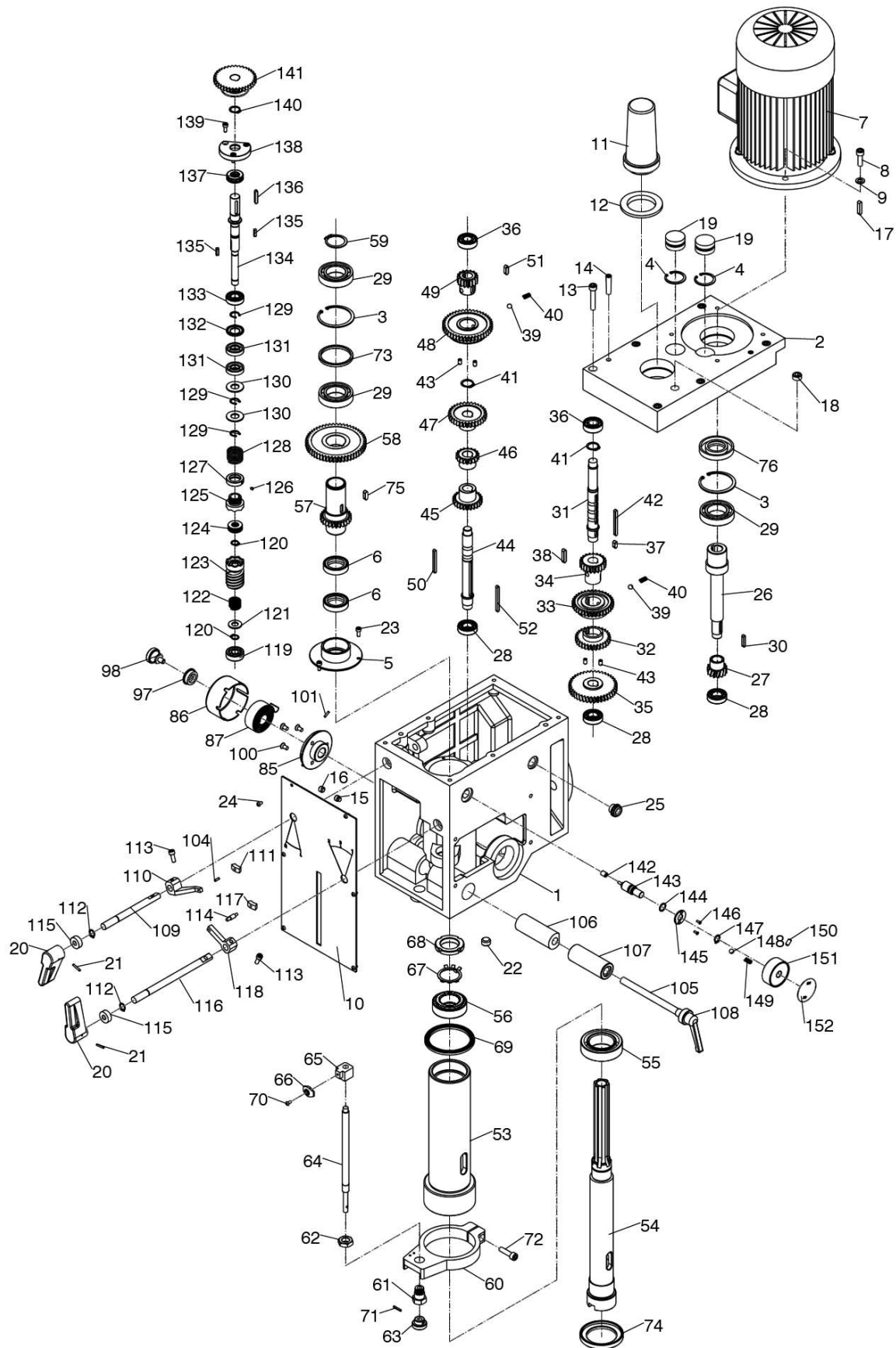
Abb.1-2: Spindelkopf - Drilling head - DH40 CTP
