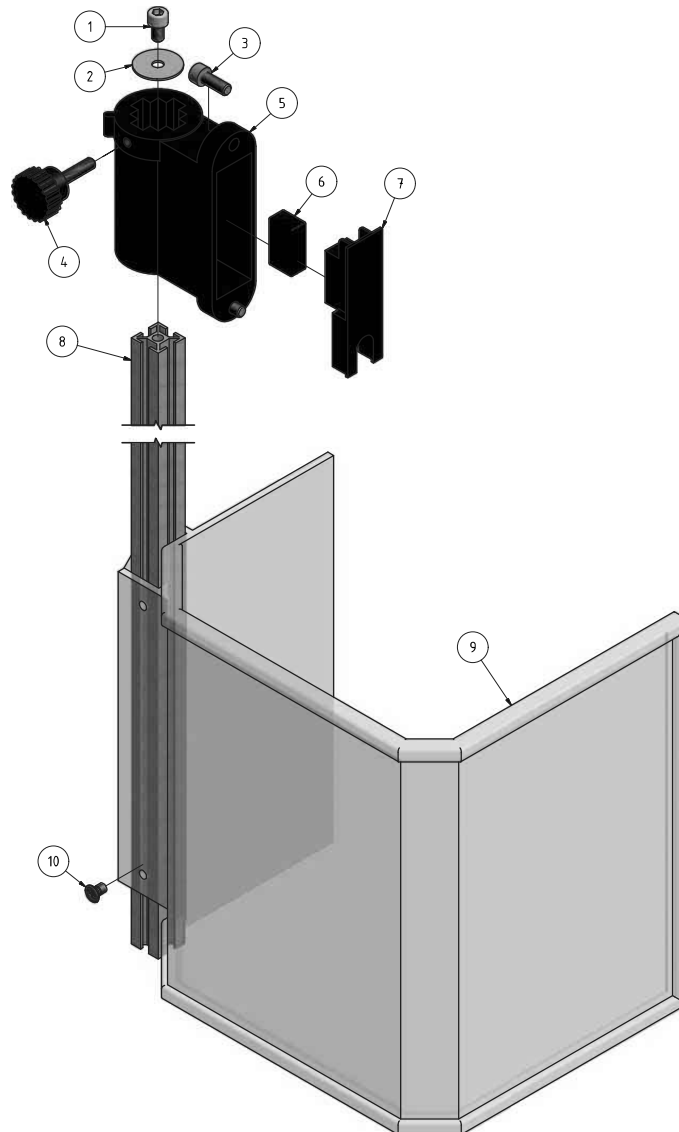
Img.1-12: Bohrfutterschutz - Drilling chuck protection
