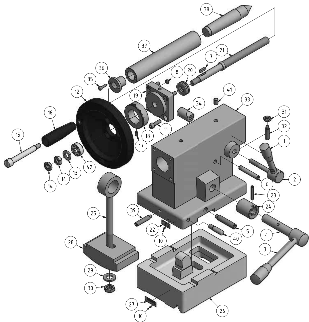
Abb.1-23: Reitstock - Tailstock
