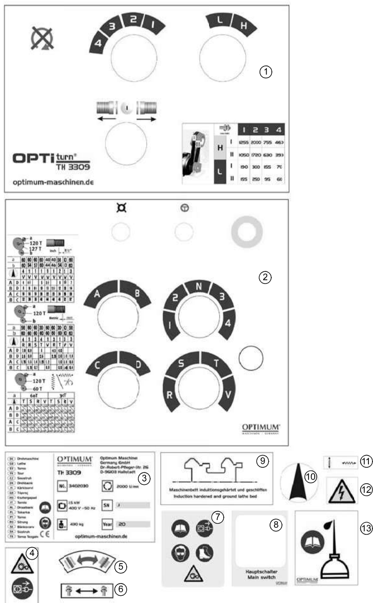
Abb. 1-28: Maschinenschilder - Machine labels
