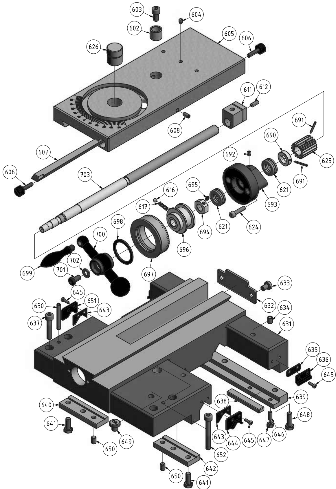
Img.1-20: Planschlitten - cross slide
