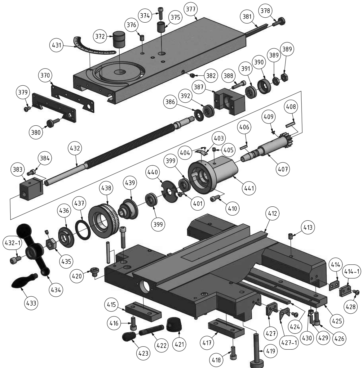
Abb.1-14: Planschlitten - Cross slide
