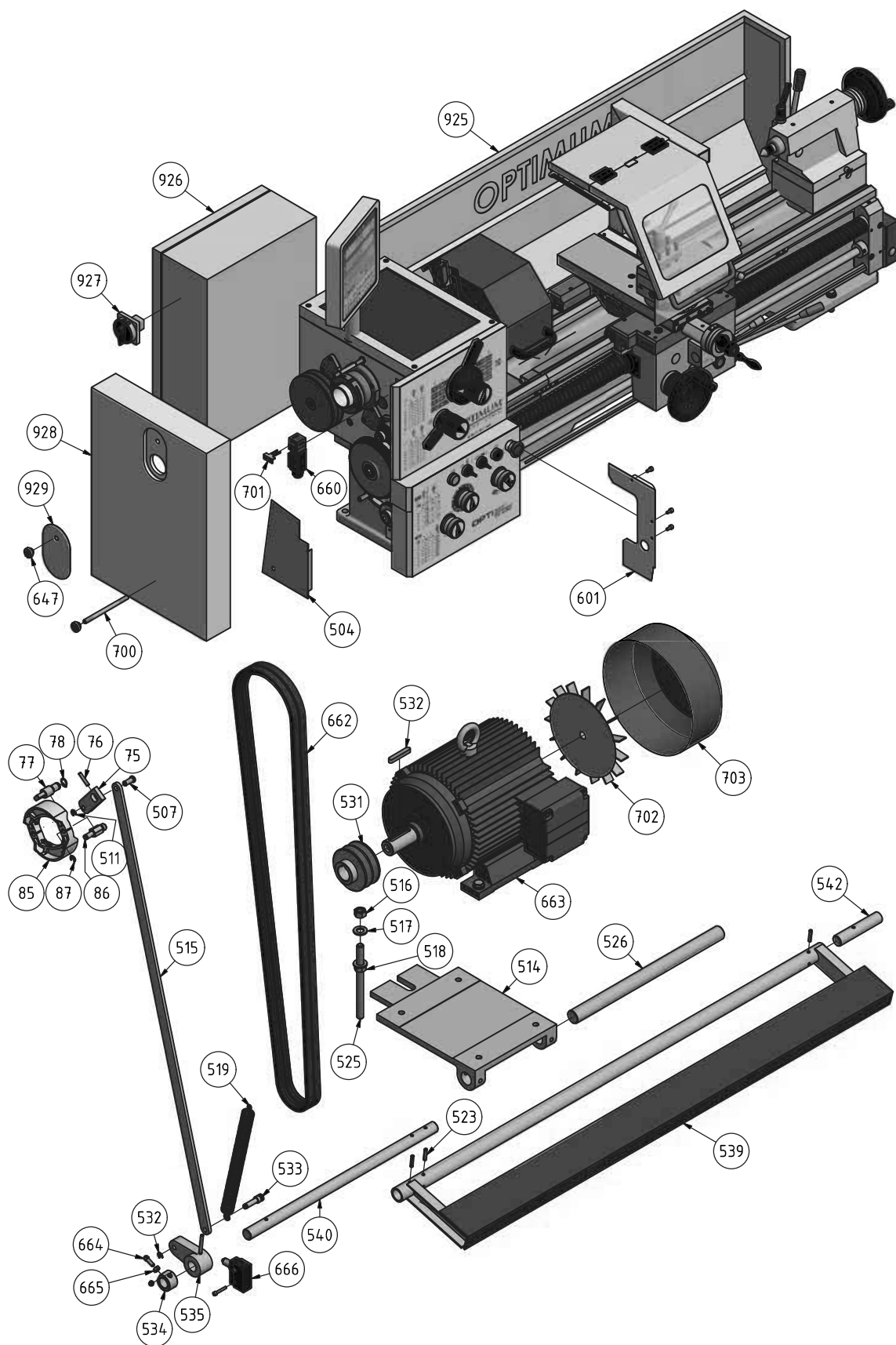
Abb. 1-19: Maschinenbett - Lathe bed
