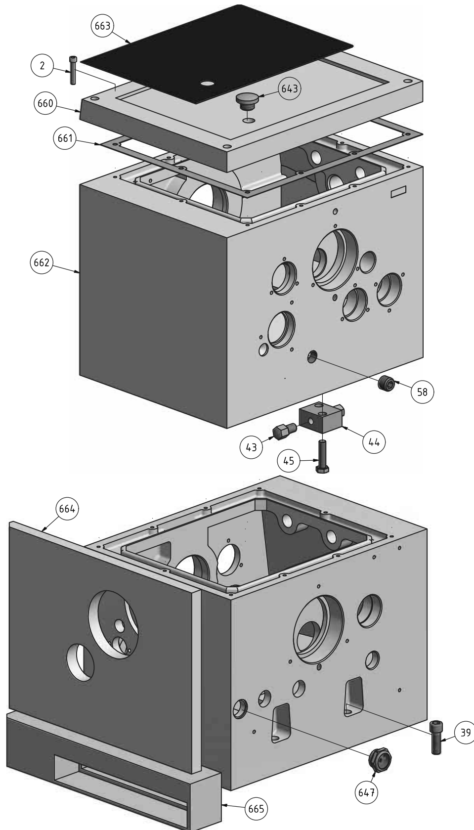
Abb. 1-1: Spindelstock - Headstock
