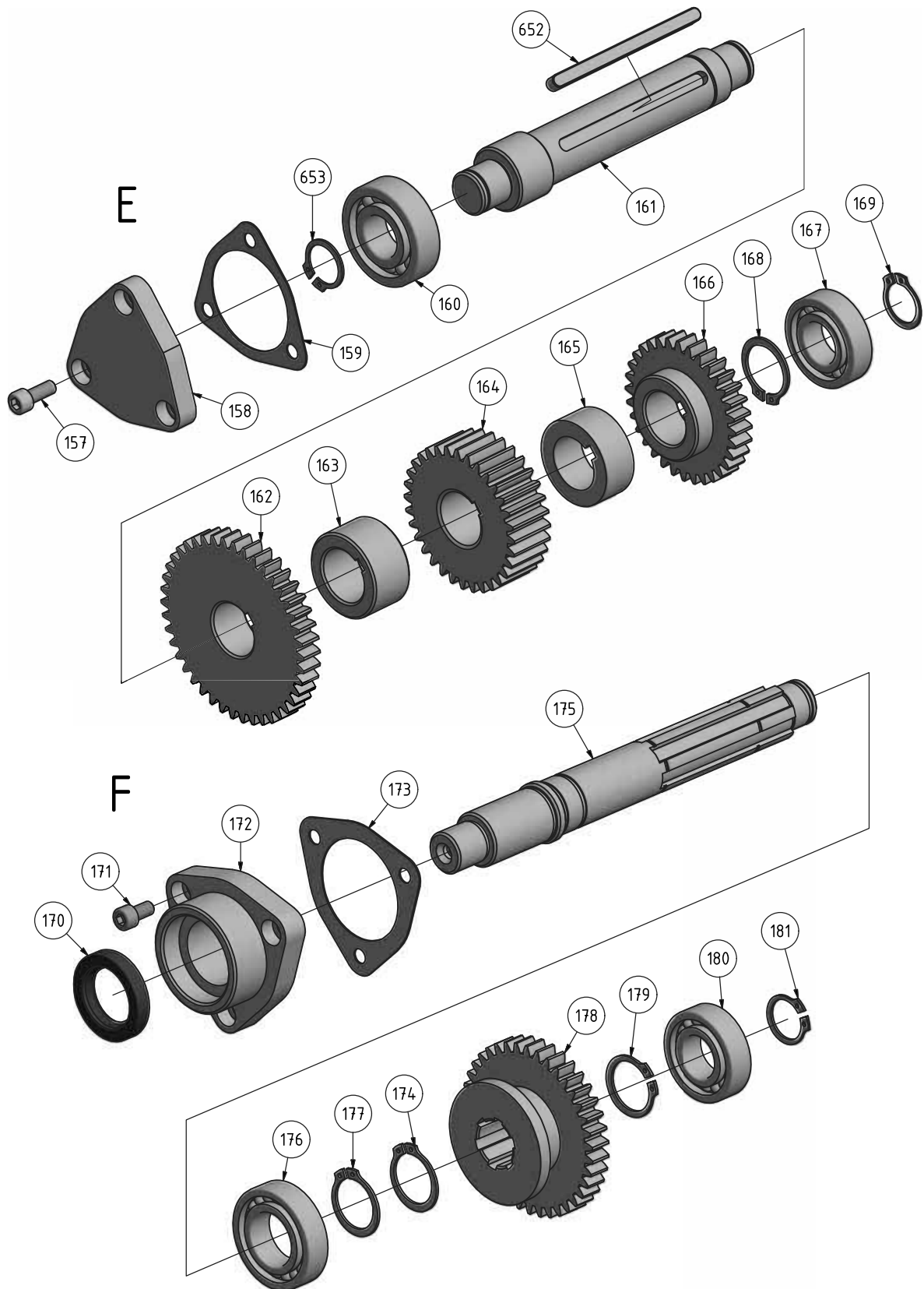
Abb.1-5: Spindelstock - Headstock
