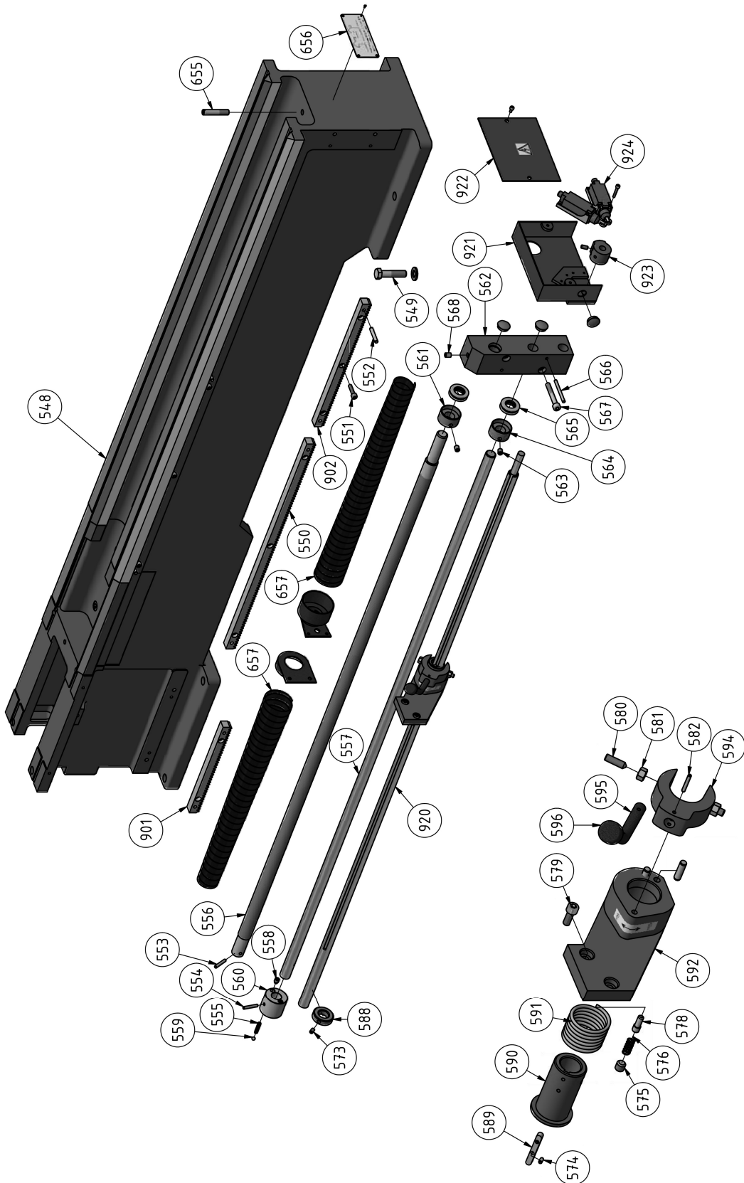
Abb.1-20: Maschinenbett - Lathe bed
