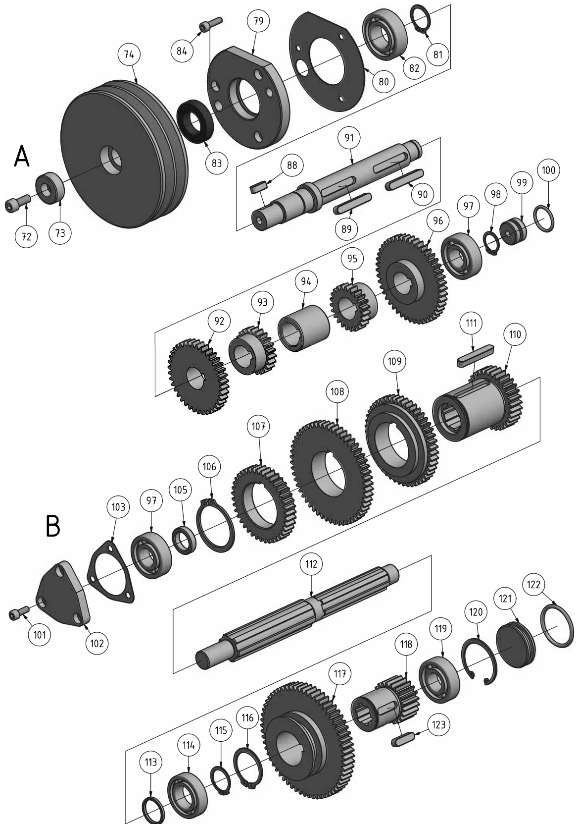
Abb. 1-3: Spindelstock - Headstock
