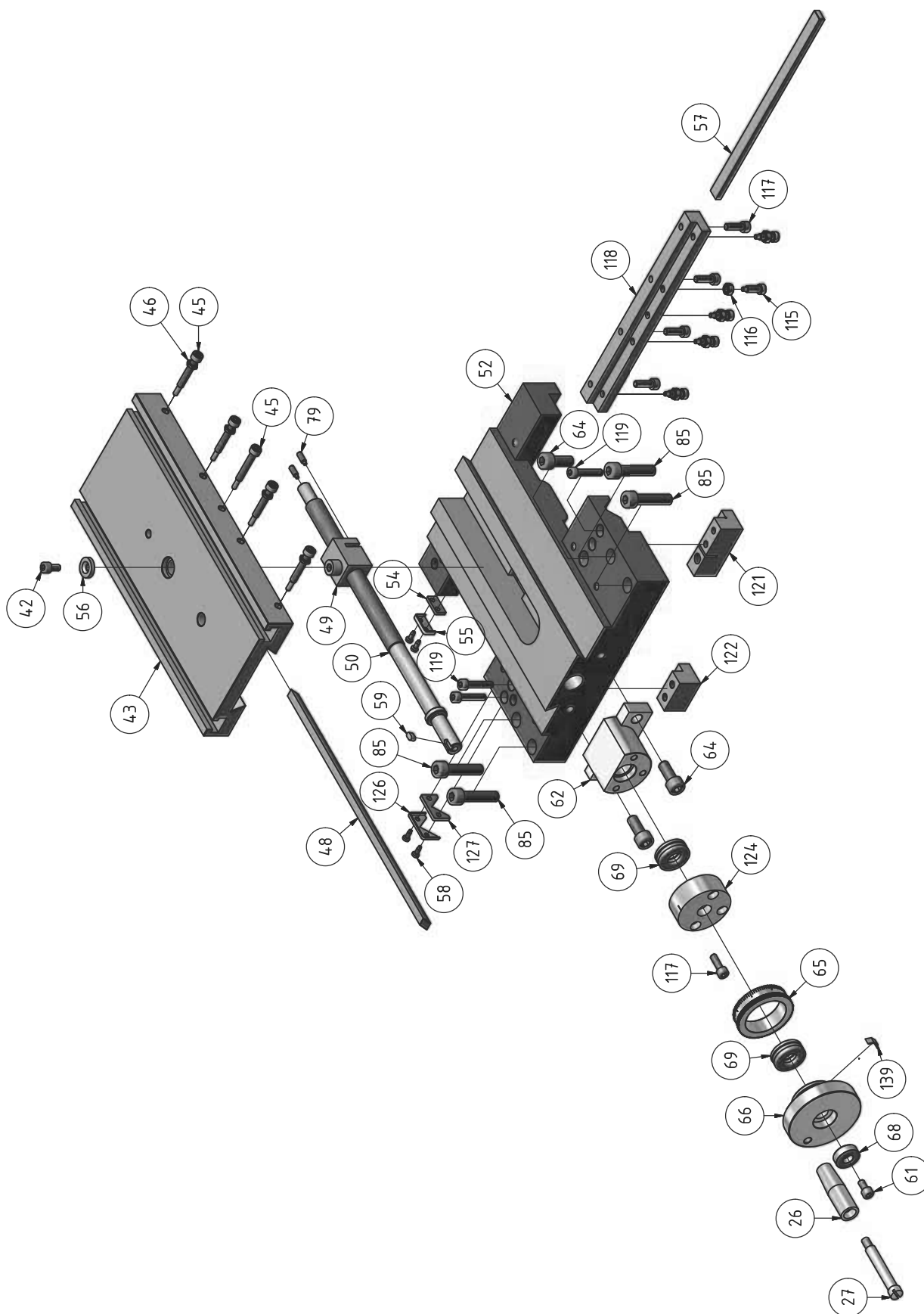
Abb. 1-2: Planschlitten - Cross slide TU 2506
