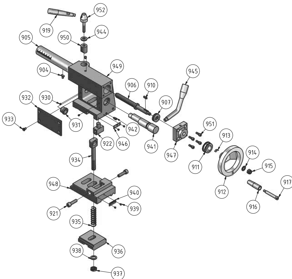
Abb. 1-4: Reitstock - Tailstock TU 2506
