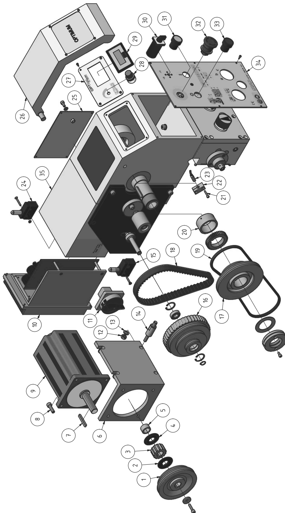
Abb.1-23: Spindelstock - Headstock TU 2807 V
