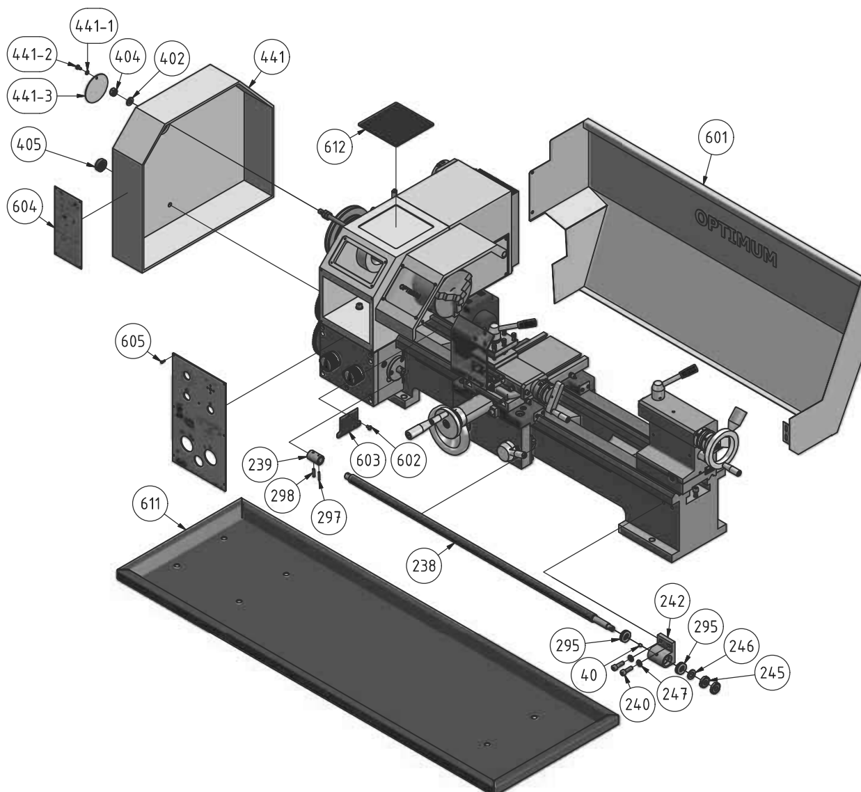
Abb. 1-18: Maschinenbett - Machine bed
