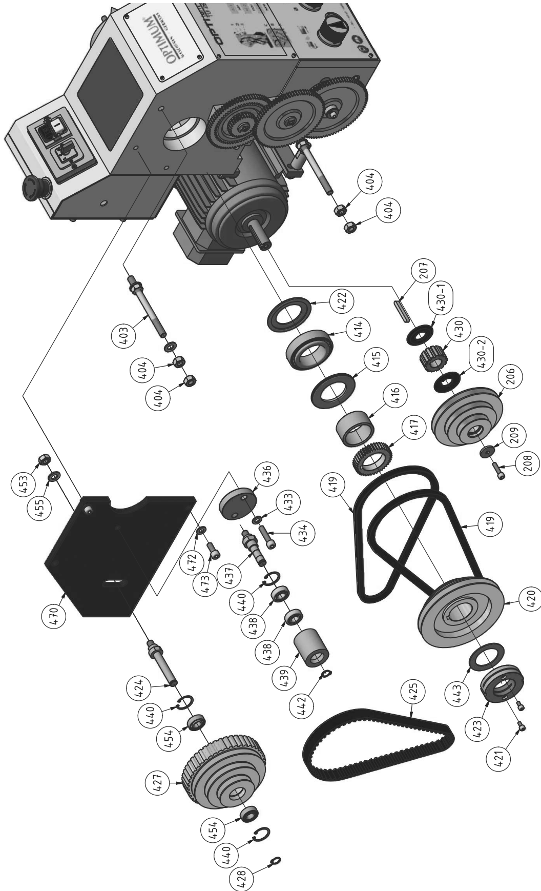
Abb.1-21: Spindelstock 1 von 2 - Headstock 1 of 2
