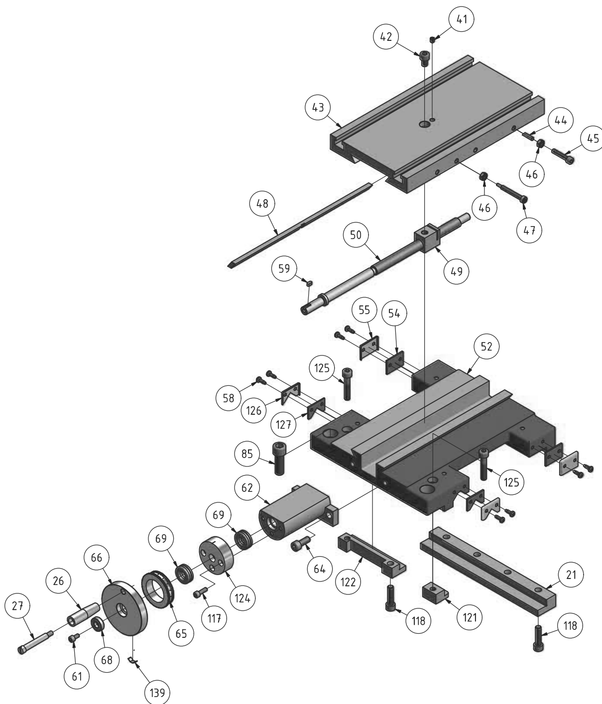
Abb. 1-15: Planschlitten - Cross slide
