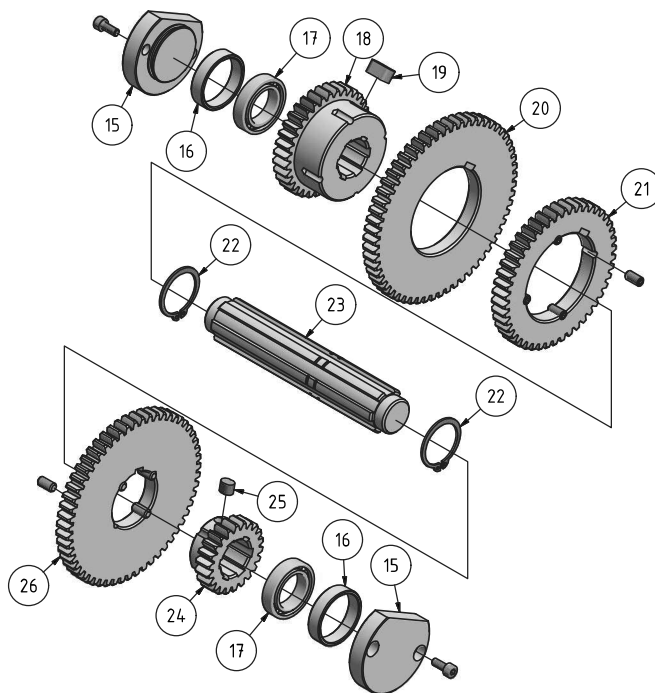
Abb. 1-1: Spindelstock - Headstock
