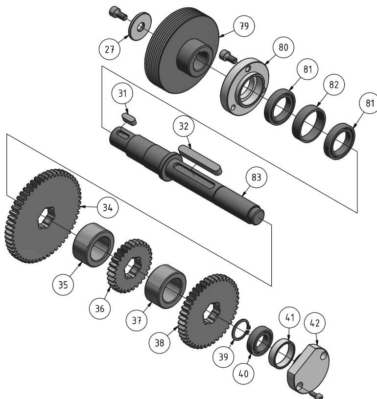
Abb. 1-3: Spindelstock - Headstock
