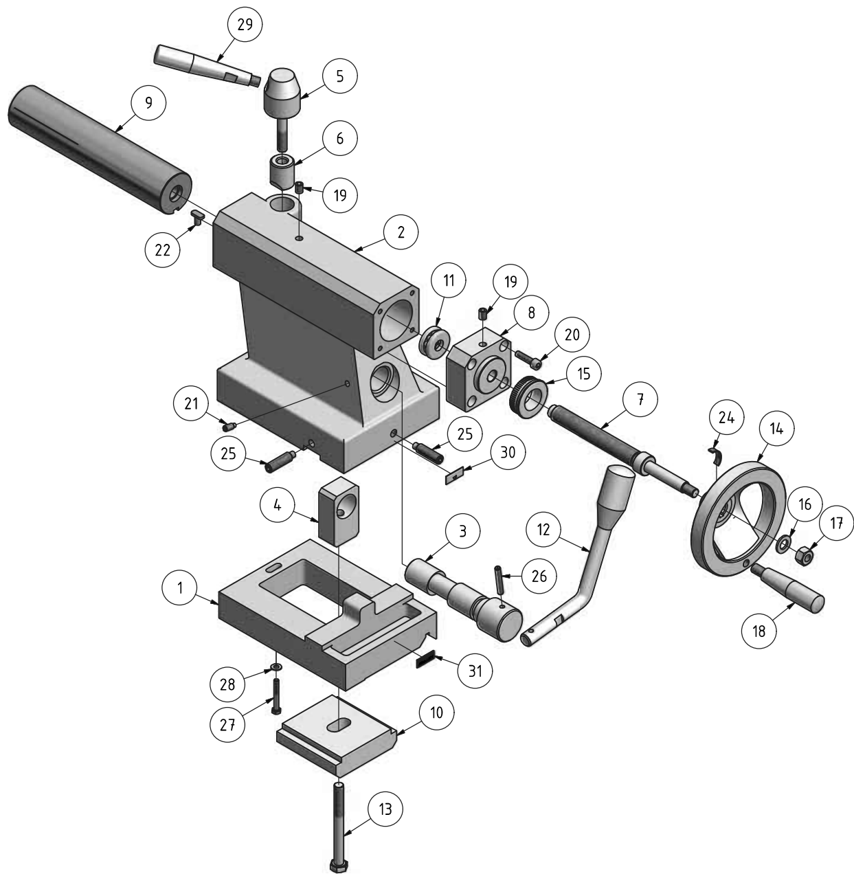
Abb. 1-14: Reitstock - Tailstock
