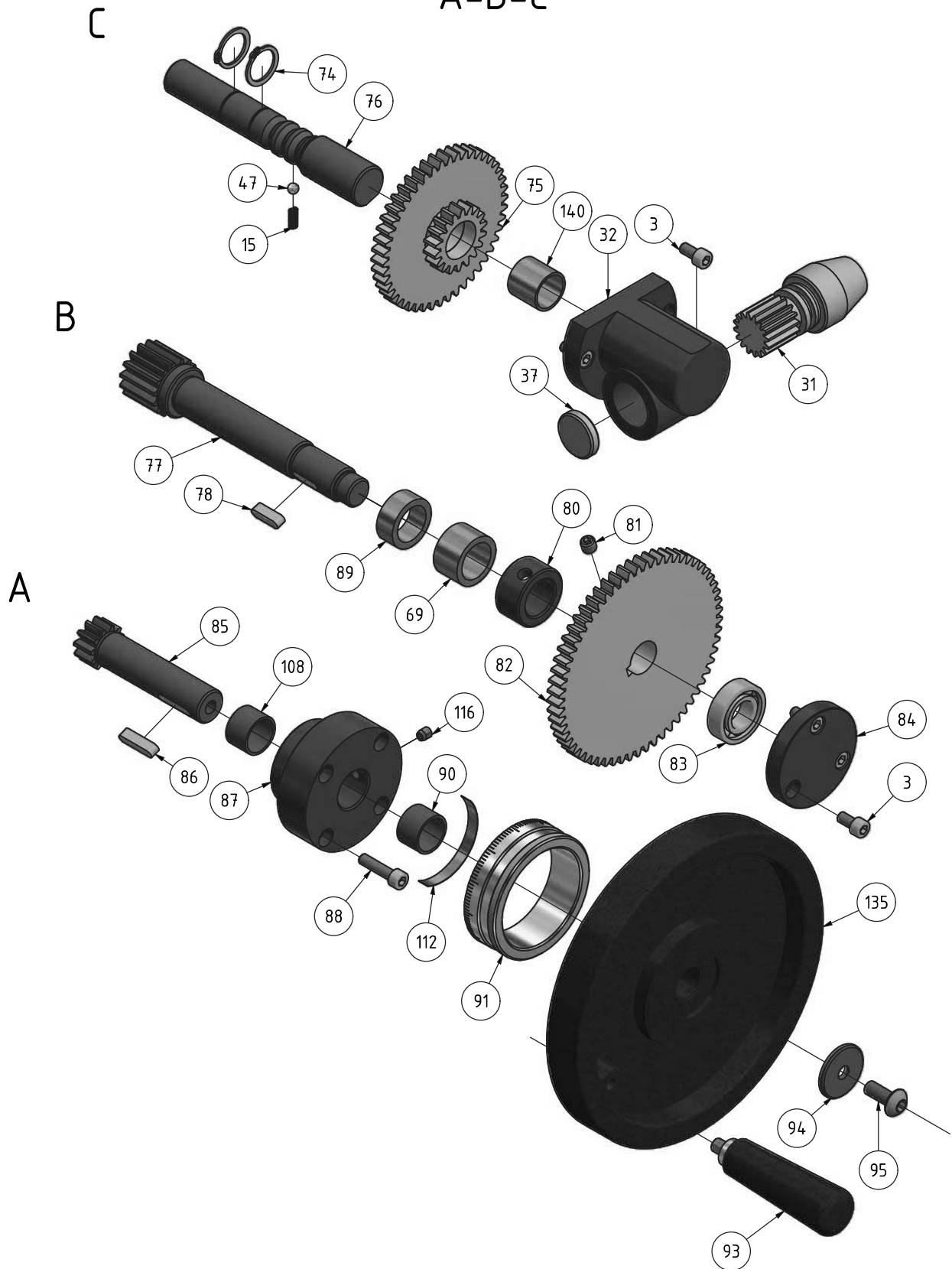
Img.1-20: Bettschlitten 2-3 - Lathe saddle 2-3
