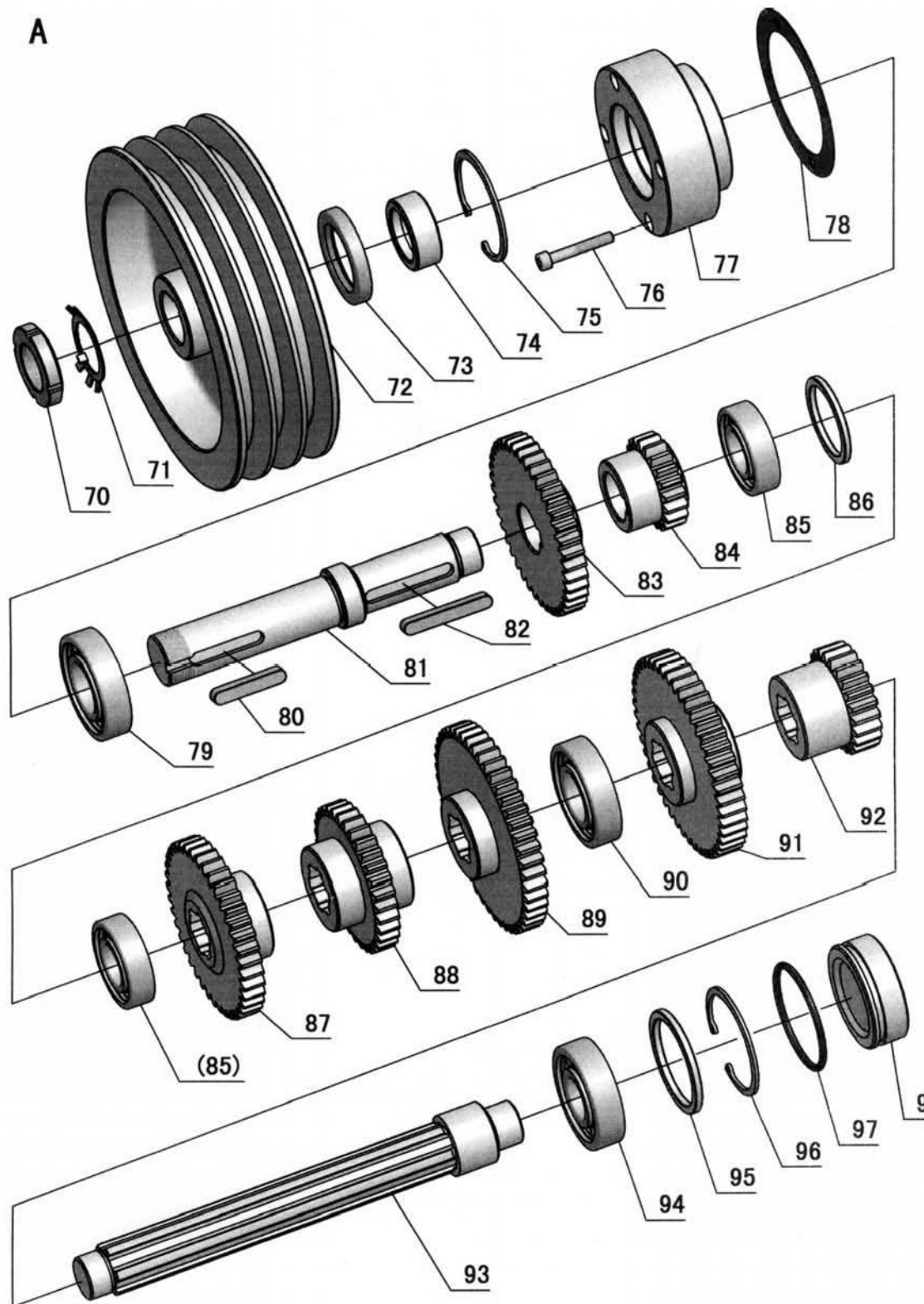
Img.1-4: Spindelstock 4 von 9 - Headstock 4 of 9
