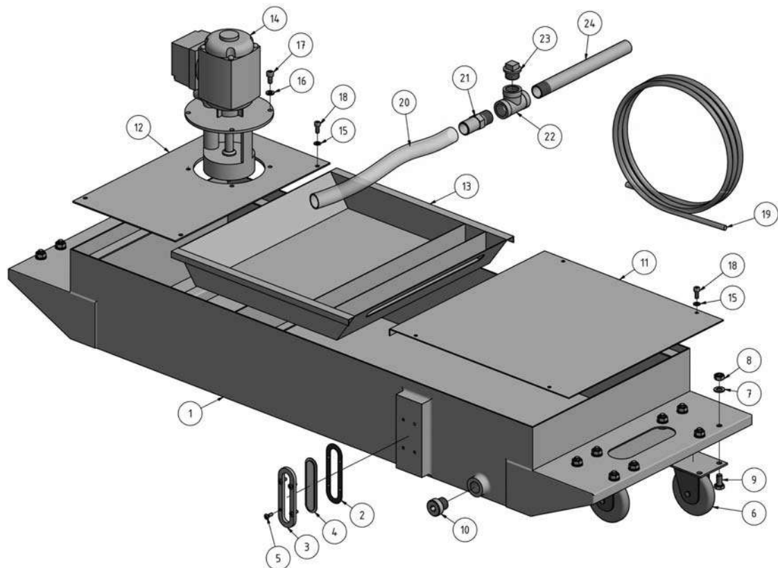
Img.1-31: Kühlmittel tank - Coolant tank
