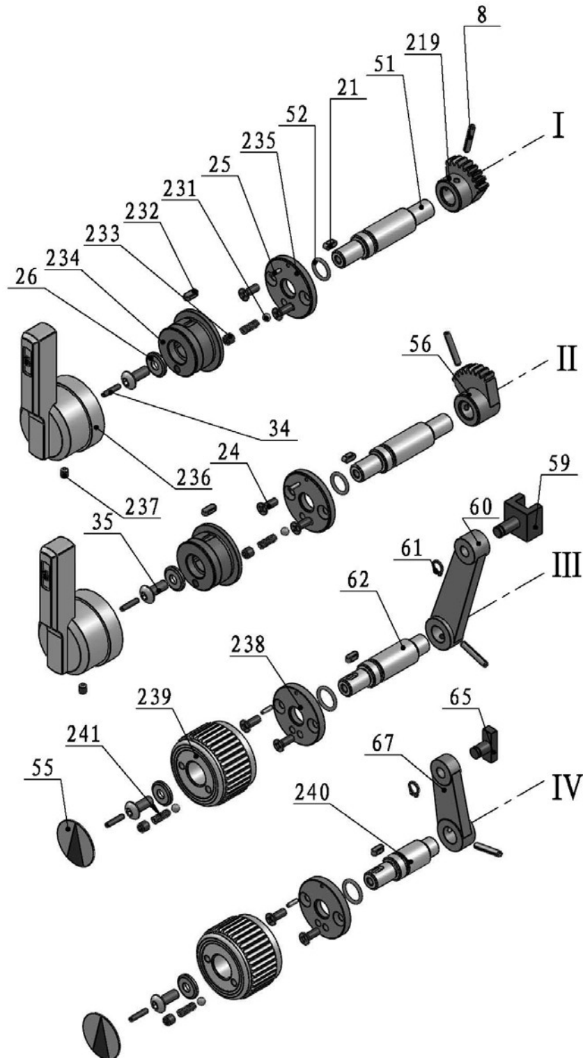
Img.1-3: Spindelstock 3 von 9 - Headstock 3 of 9
