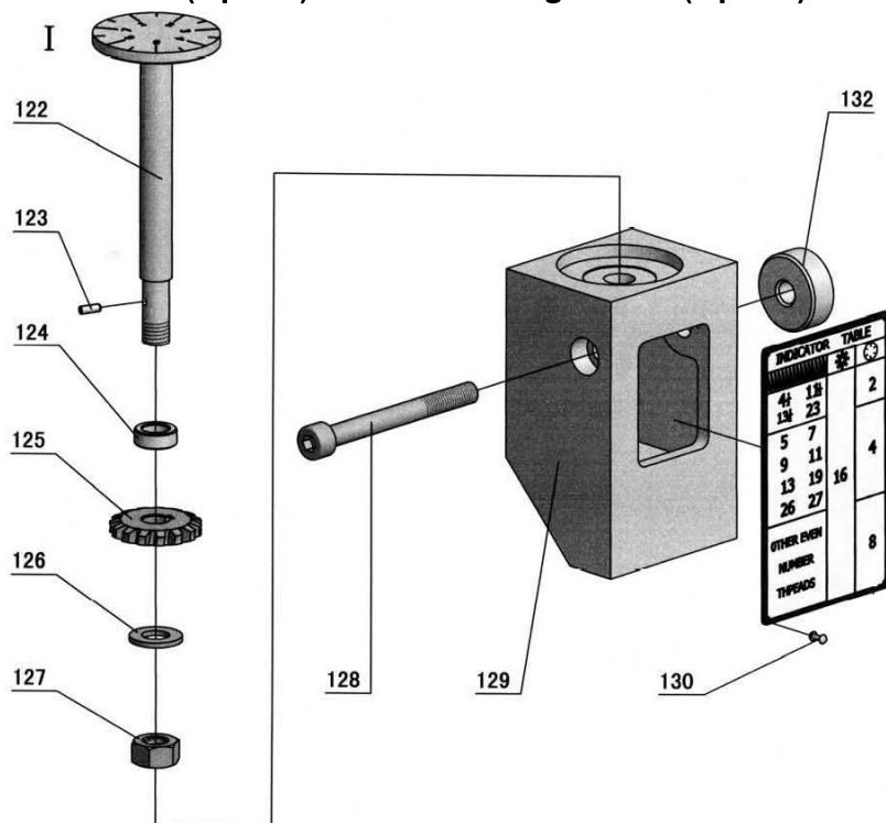
Img.1-19: Gewindeuhr - Thread cutting device
