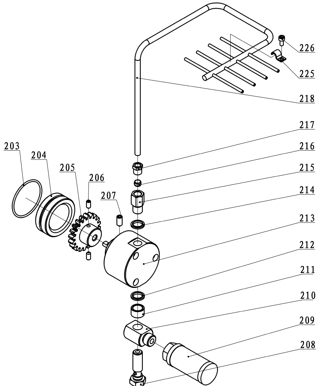
Img. 1-9: Spindelstock 9 von 9 - Headstock 9 of 9
