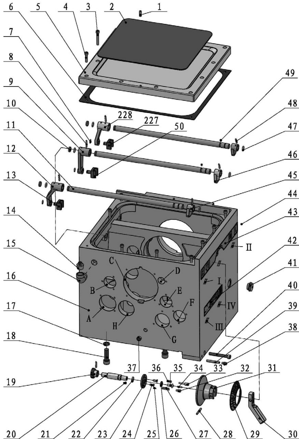
Img.1-1: Spindelstock 1 von 9 - Headstock 1 of 9
