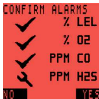
Figure 6-7: Confirm Alarms - Fails
