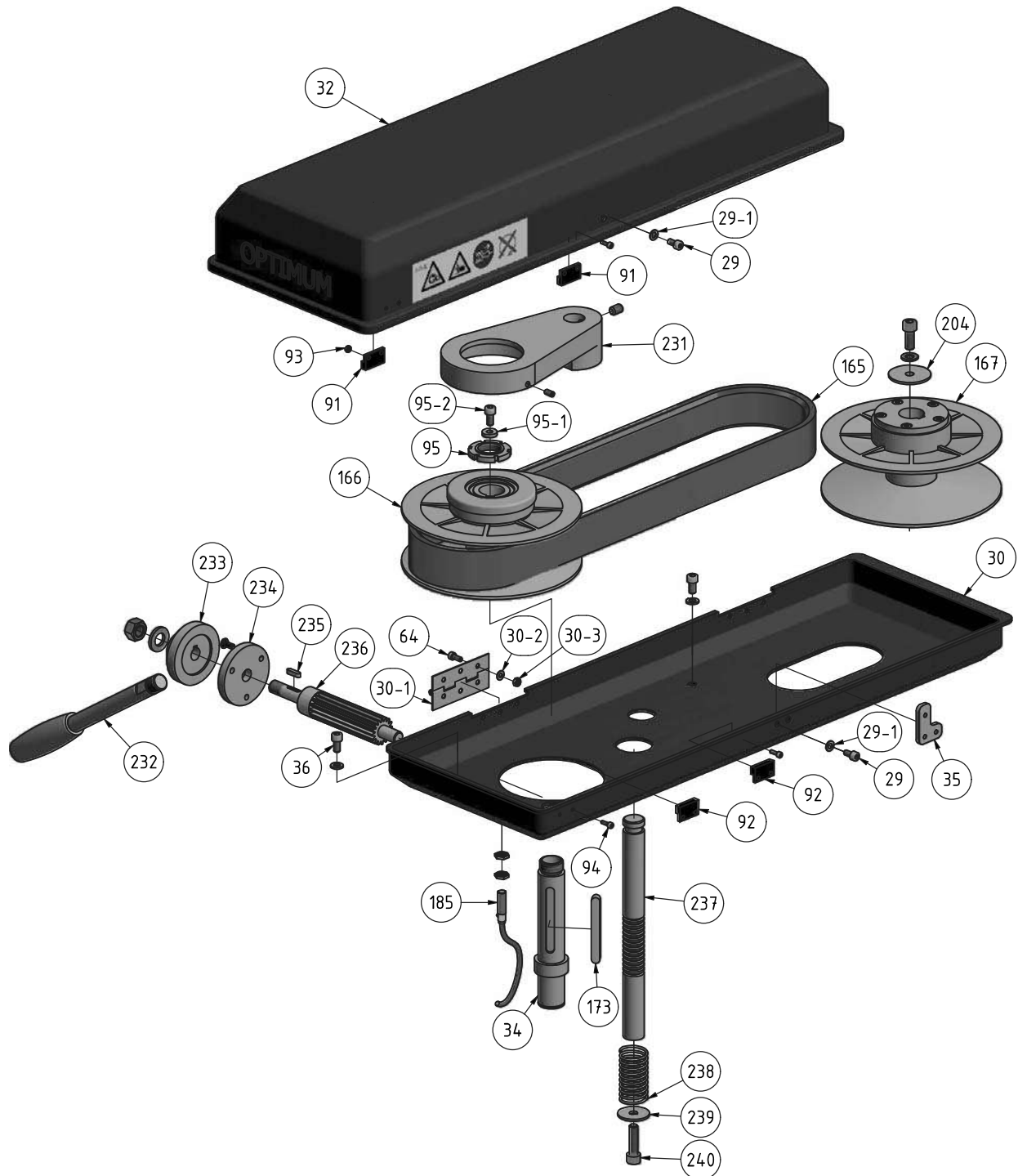
Abb.1-5: Antrieb DH24BV - Drive DH24BV
