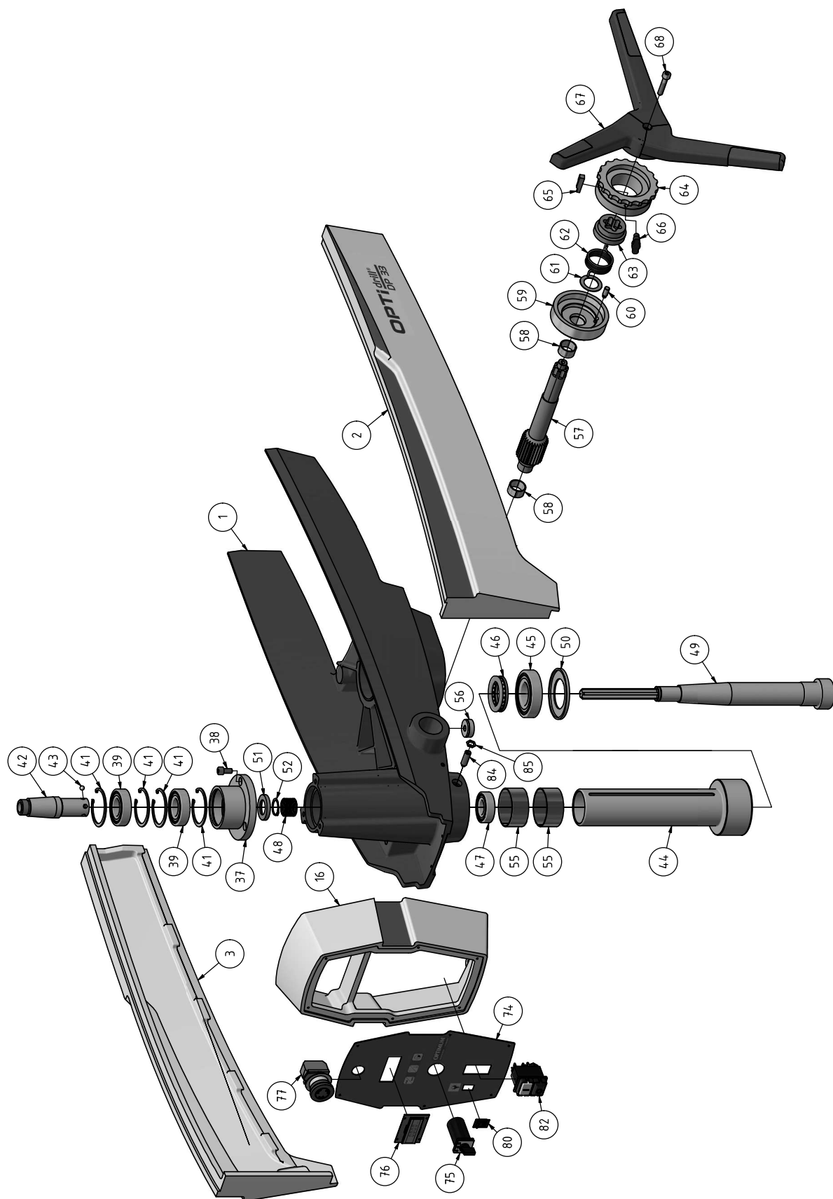
Abb. 1-2: Bohrkopf - Drilling head
