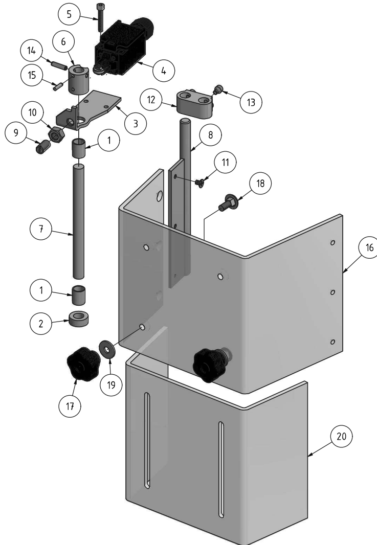
Abb. 1-4: Bohrfutterschutz - Drill chuck guard
