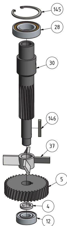
Img.0-5: Bohrkopf - Drilling head
