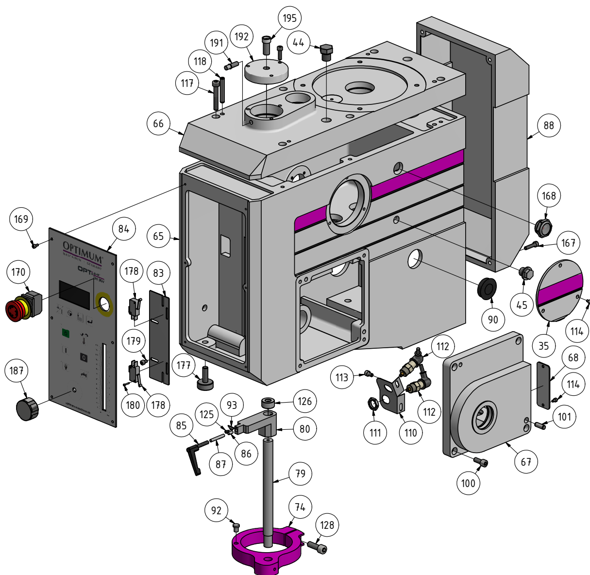
Img.0-7: Bohrkopf - Drilling head
