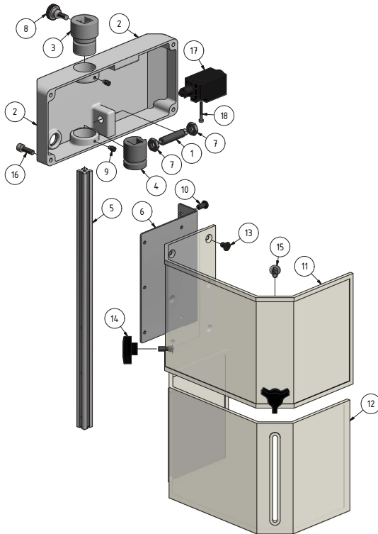
Img.0-9: Bohrfutterschutz- Drill chuck protection
